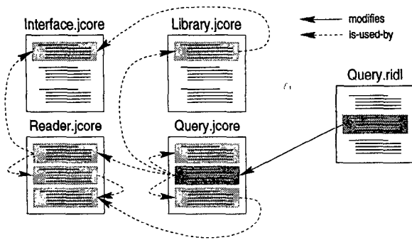
Figure 5: Non-localized Semantic Analysis with Rid1
