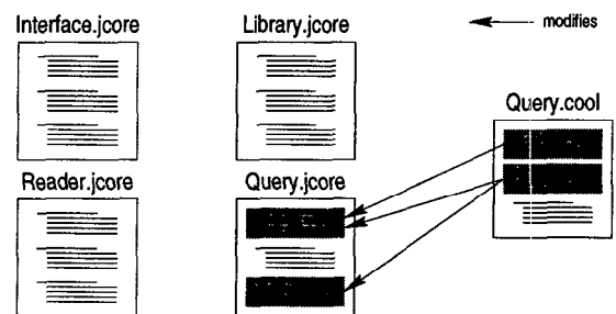
Figure 4: Localized Semantic Analysis with Cool
